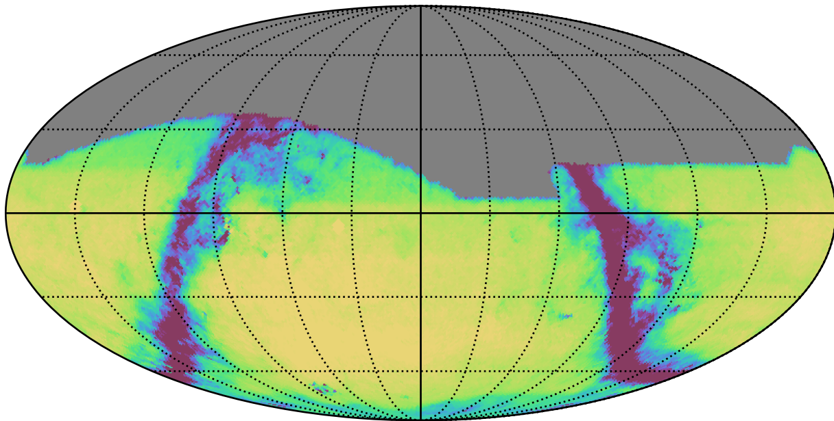
too_elab_r32_d2_giz_v3.4_10yrs All sky g band: Exgal_CoaddM5
