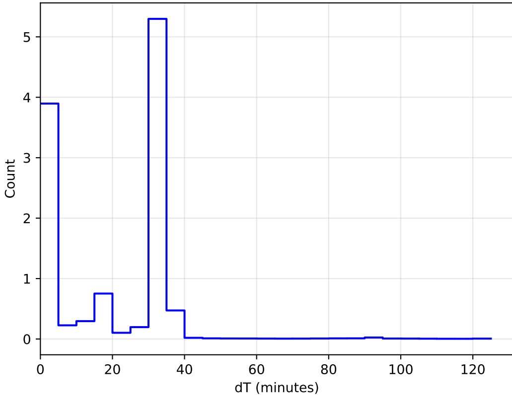
too_elab_r32_d2_giz_v3.4_10yrs WFD: DeltaT Histogram
