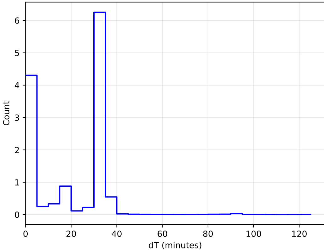
too_elab_r32_d2_giz_v3.4_10yrs All sky: DeltaT Histogram 1e6
