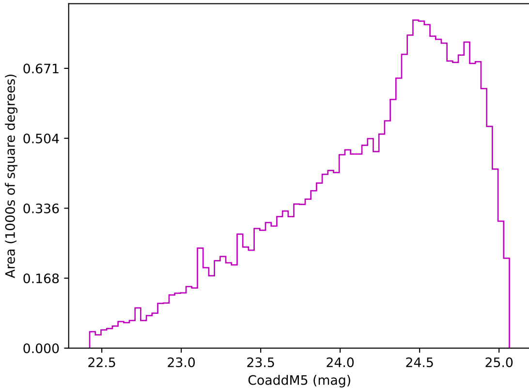
too_elab_r32_d2_giz_v3.4_10yrs Yr 3-4 z band: CoaddM5
