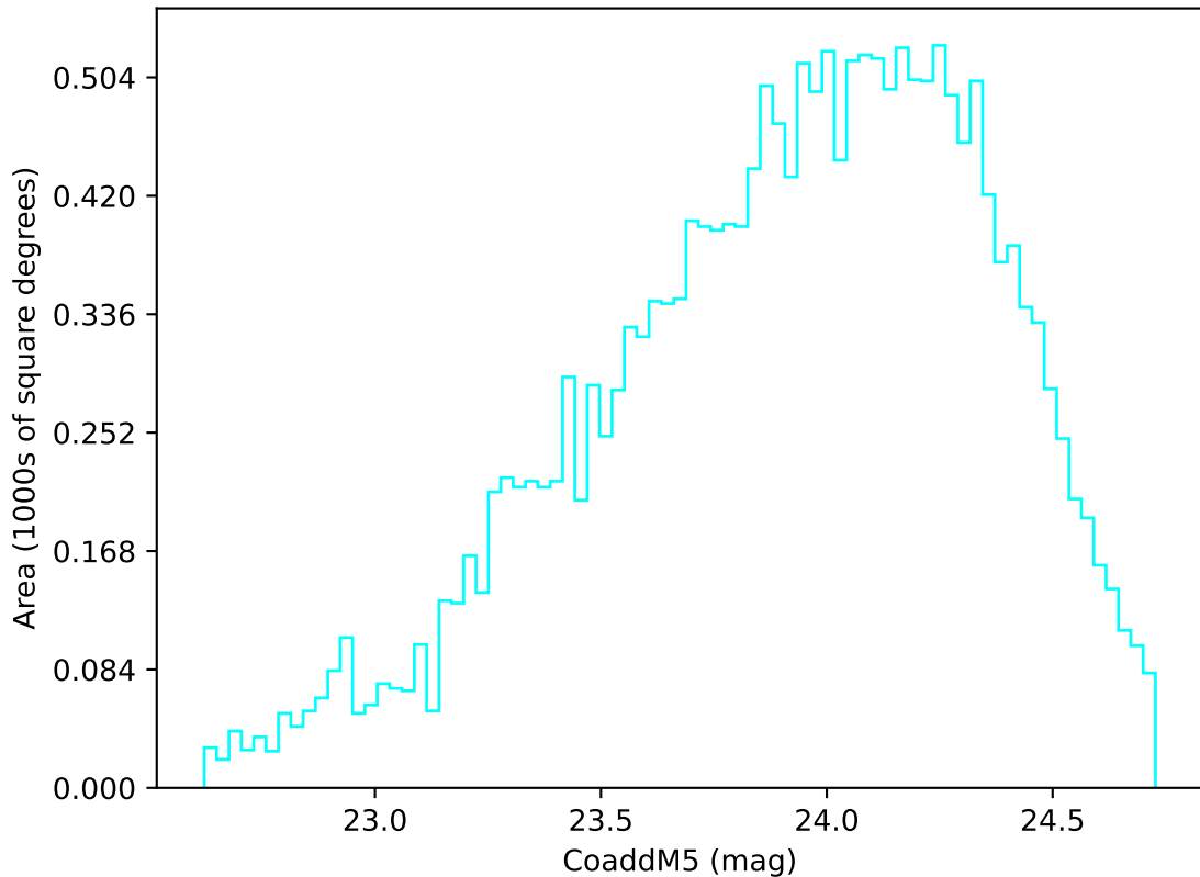
too_elab_r32_d2_giz_v3.4_10yrs Yr 3-4 u band: CoaddM5
