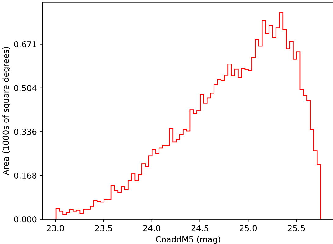
too_elab_r32_d2_giz_v3.4_10yrs Yr 3-4 i band: CoaddM5
