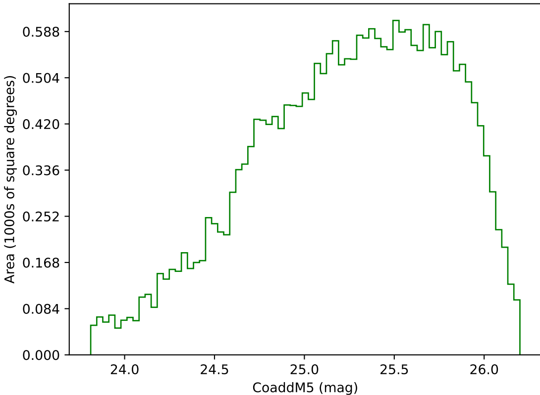
too_elab_r32_d2_giz_v3.4_10yrs Yr 3-4 g band: CoaddM5
