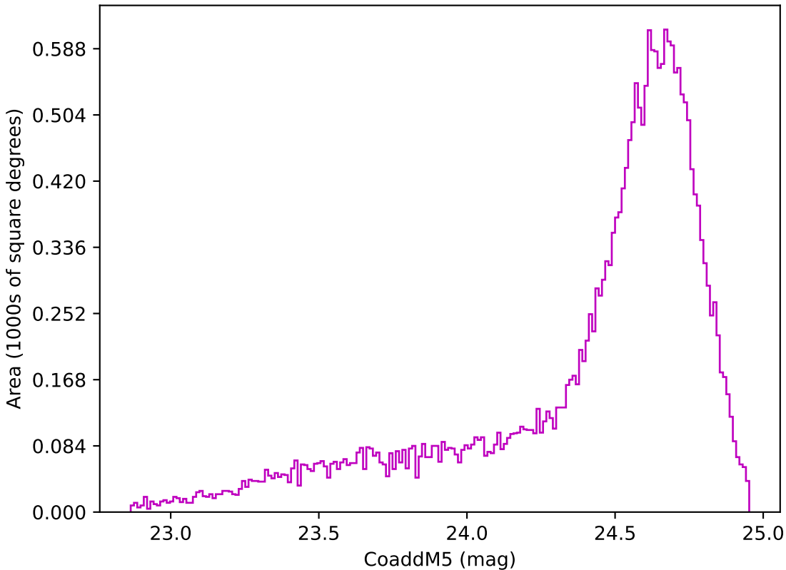
too_elab_r32_d2_giz_v3.4_10yrs Yr 1 z band: CoaddM5
