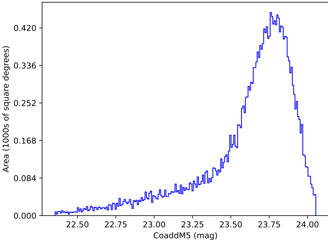
too_elab_r32_d2_giz_v3.4_10yrs Yr 1 y band: CoaddM5
