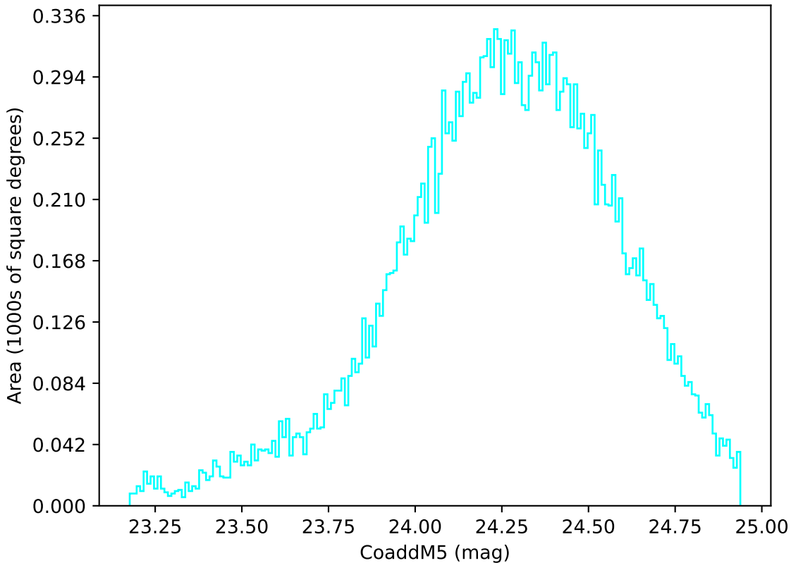
too_elab_r32_d2_giz_v3.4_10yrs Yr 1 u band: CoaddM5
