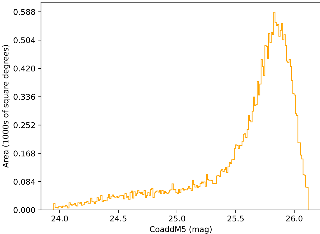
too_elab_r32_d2_giz_v3.4_10yrs Yr 1 r band: CoaddM5
