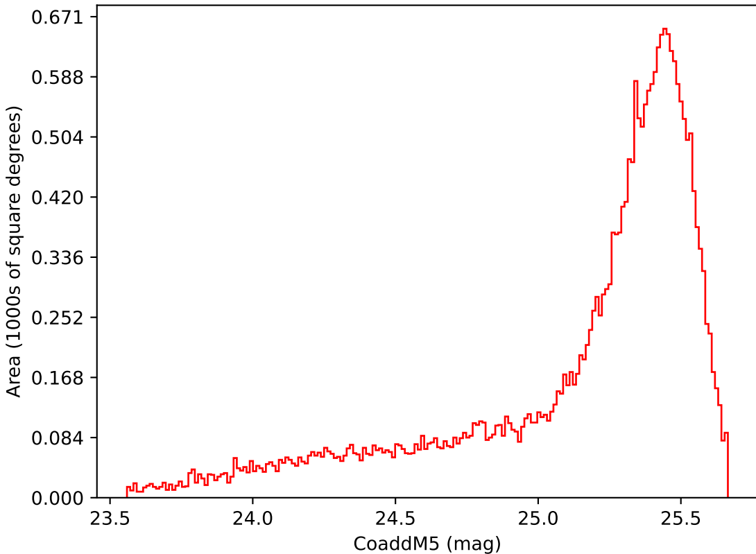
too_elab_r32_d2_giz_v3.4_10yrs Yr 1 i band: CoaddM5
