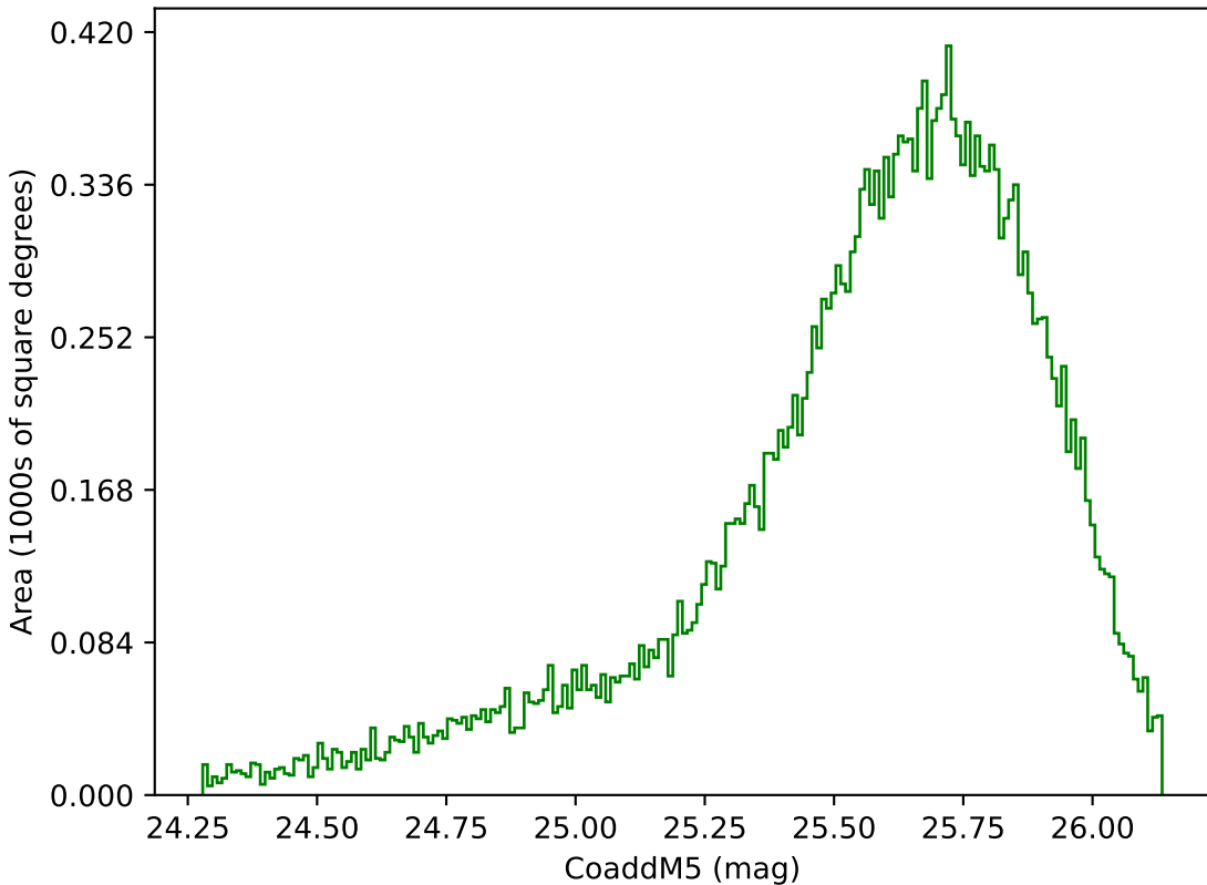
too_elab_r32_d2_giz_v3.4_10yrs Yr 1 g band: CoaddM5
