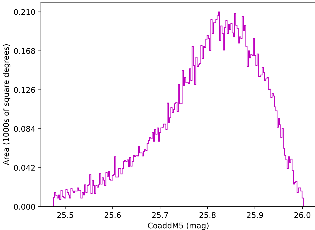
too_elab_r32_d2_giz_v3.4_10yrs WFD z band: CoaddM5
