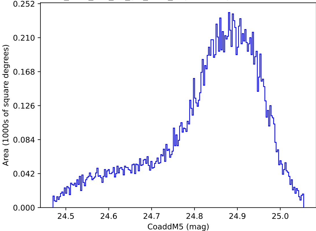
too_elab_r32_d2_giz_v3.4_10yrs WFD y band: CoaddM5
