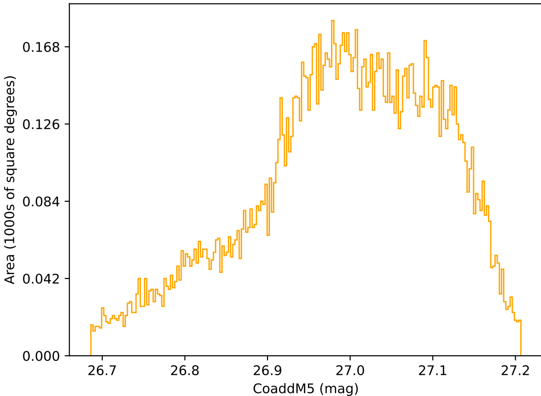
too_elab_r32_d2_giz_v3.4_10yrs WFD r band: CoaddM5
