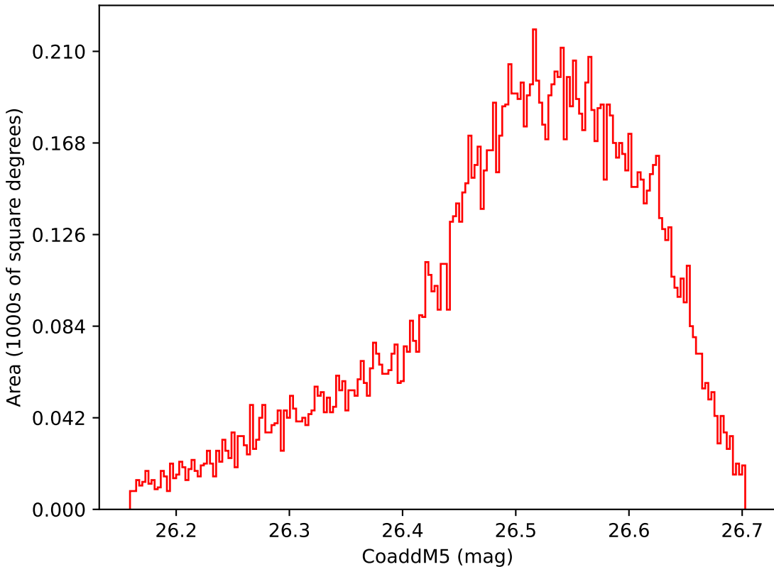
too_elab_r32_d2_giz_v3.4_10yrs WFD i band: CoaddM5
