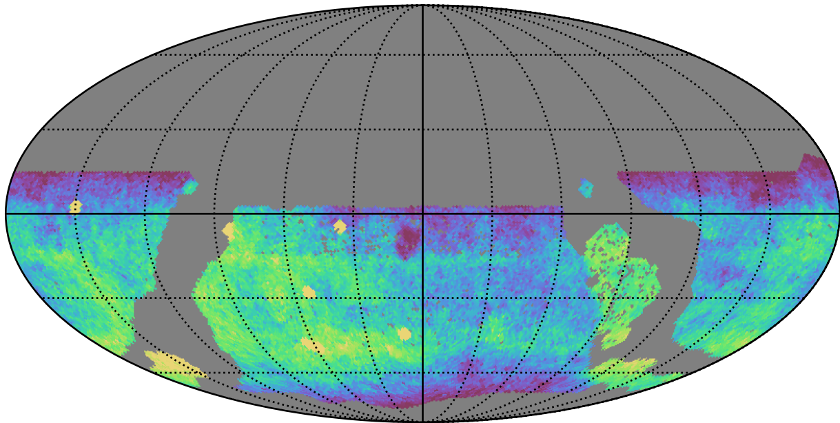
too_elab_r32_d2_giz_v3.4_10yrs WFD g band: CoaddM5
