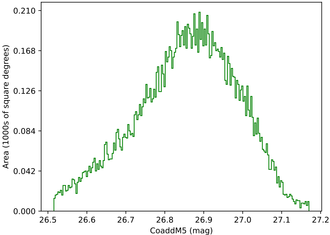
too_elab_r32_d2_giz_v3.4_10yrs WFD g band: CoaddM5
