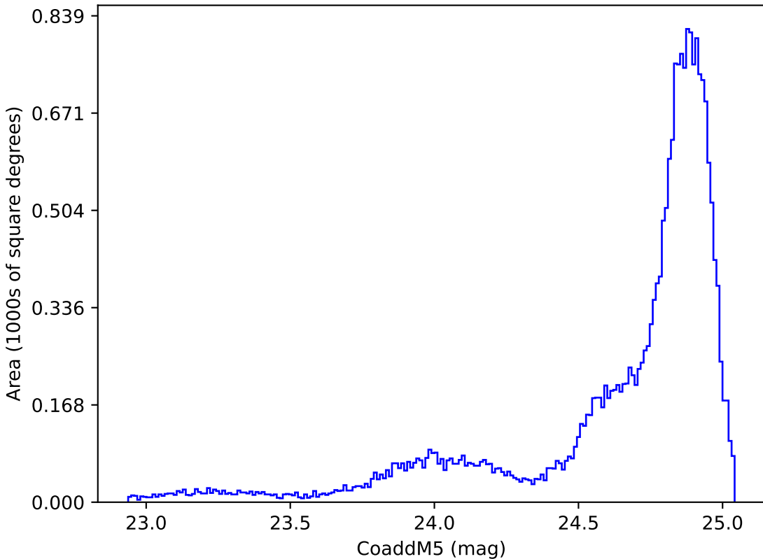
too_elab_r32_d2_giz_v3.4_10yrs All sky y band: CoaddM5
