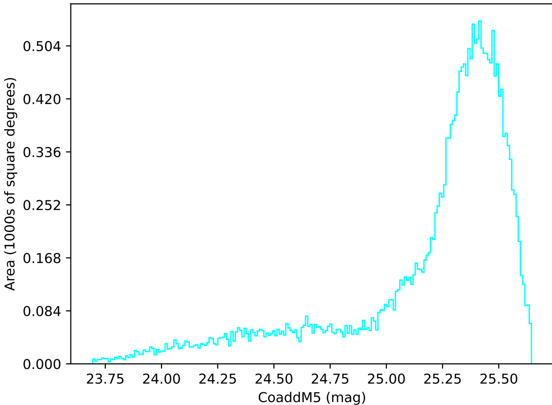
too_elab_r32_d2_giz_v3.4_10yrs All sky u band: CoaddM5
