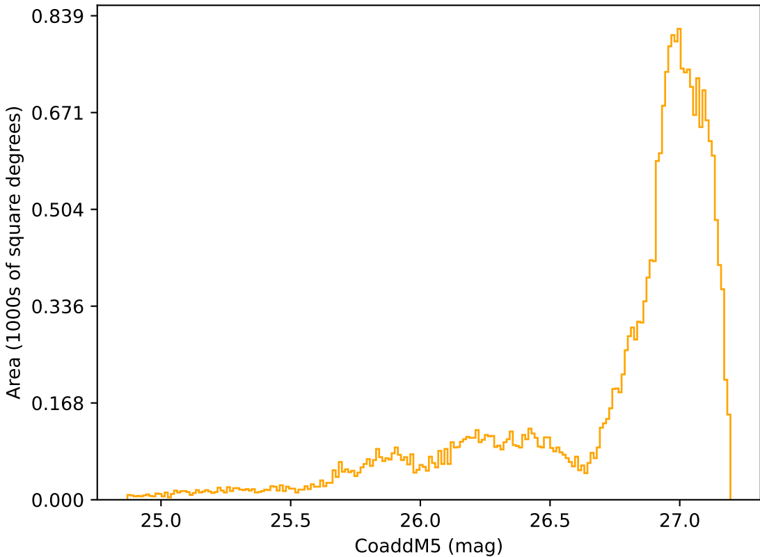
too_elab_r32_d2_giz_v3.4_10yrs All sky r band: CoaddM5
