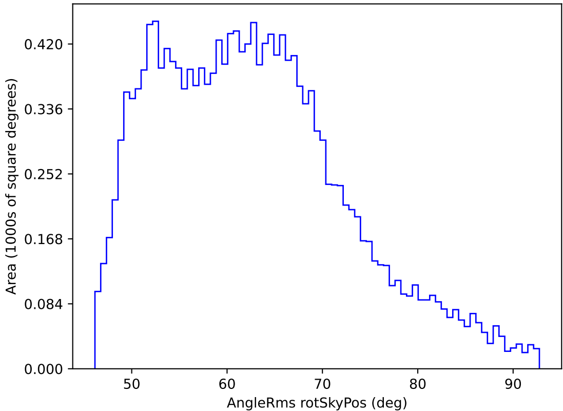
too_elab_r32_d2_giz_v3.4_10yrs WFD y band: AngleRms rotSkyPos
