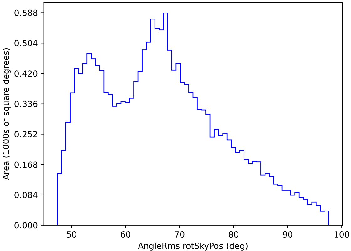
too_elab_r32_d2_giz_v3.4_10yrs WFD r band: AngleRms rotSkyPos
