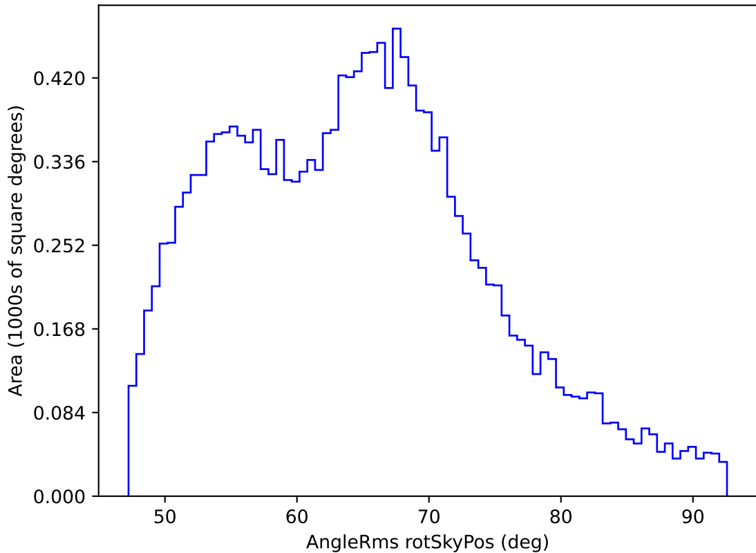
too_elab_r32_d2_giz_v3.4_10yrs WFD i band: AngleRms rotSkyPos
