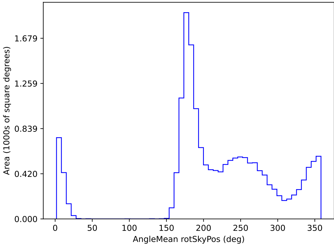
too_elab_r32_d2_giz_v3.4_10yrs WFD y band: AngleMean rotSkyPos
