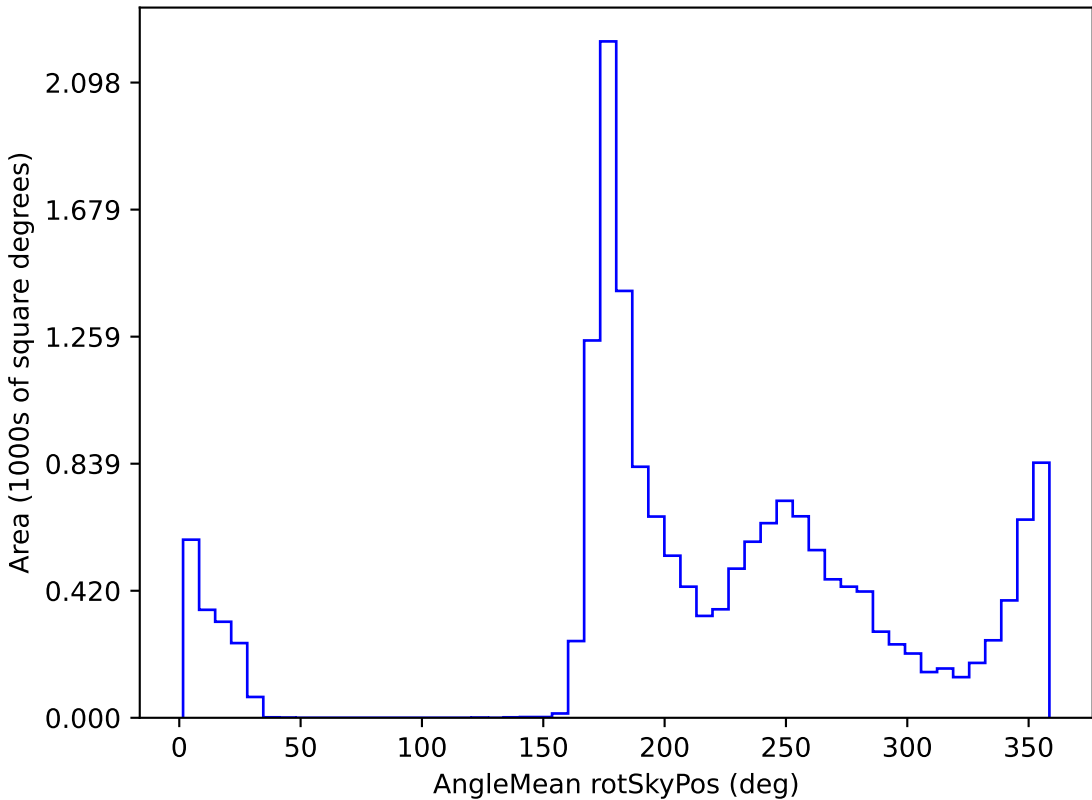
too_elab_r32_d2_giz_v3.4_10yrs WFD i band: AngleMean rotSkyPos
