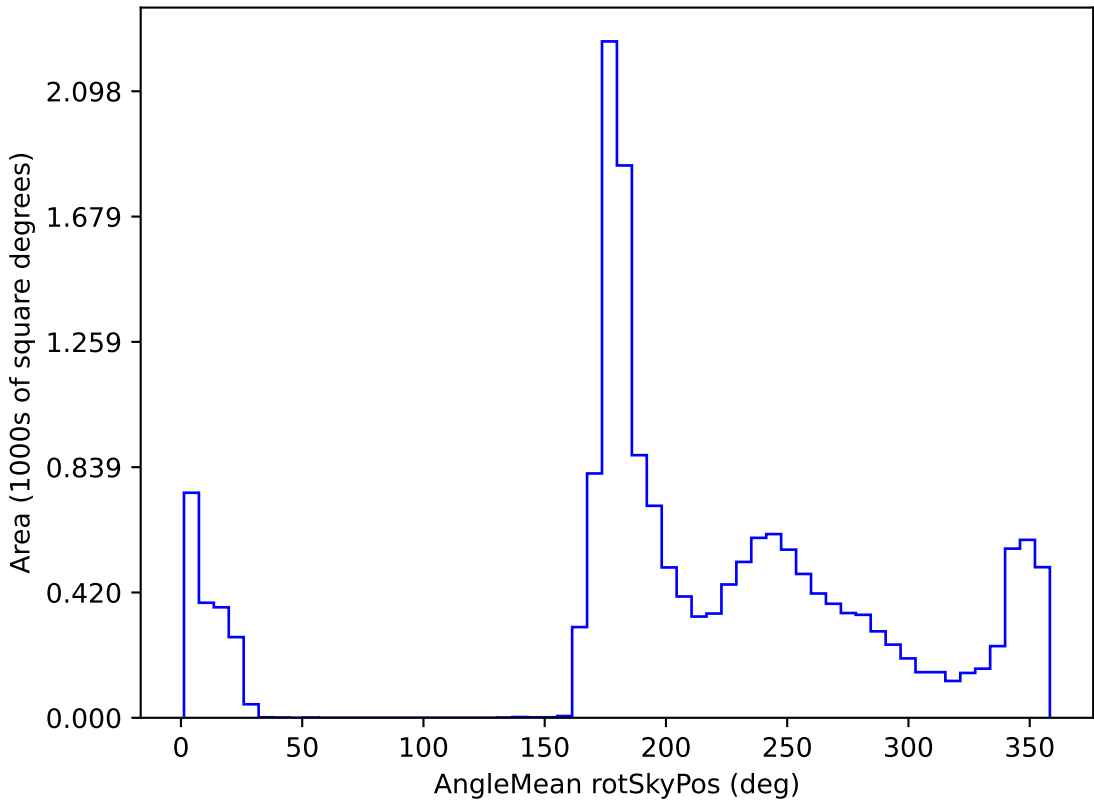
too_elab_r32_d2_giz_v3.4_10yrs WFD all bands: AngleMean rotSkyPos
