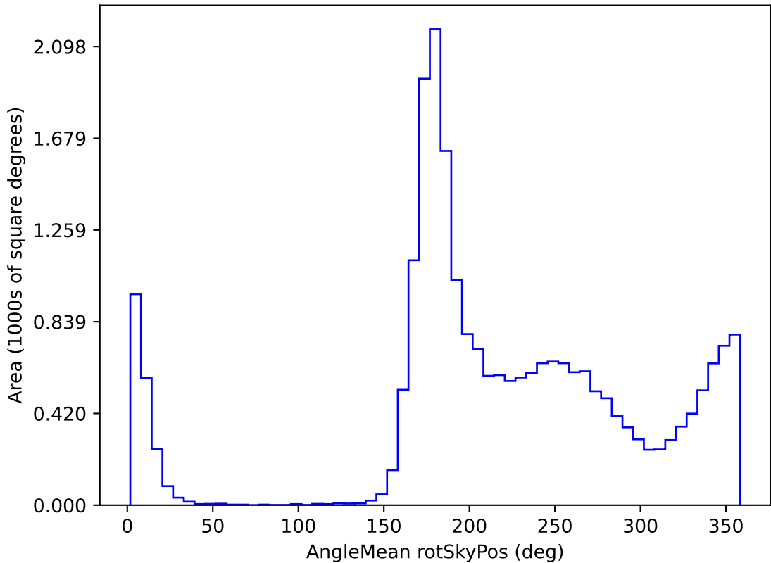
too_elab_r32_d2_giz_v3.4_10yrs All sky y band: AngleMean rotSkyPos
