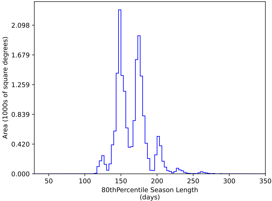
too_elab_r32_d2_giz_v3.4_10yrs WFD y band: 80thPercentile Season Length
