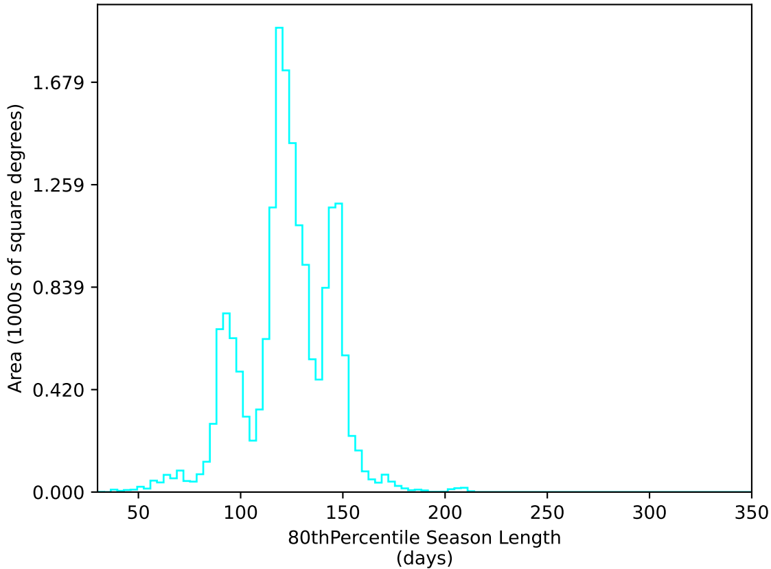
too_elab_r32_d2_giz_v3.4_10yrs WFD u band: 80thPercentile Season Length
