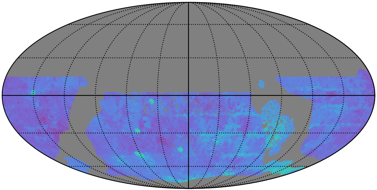
too_elab_r32_d2_giz_v3.4_10yrs WFD g band: 80thPercentile Season Length
