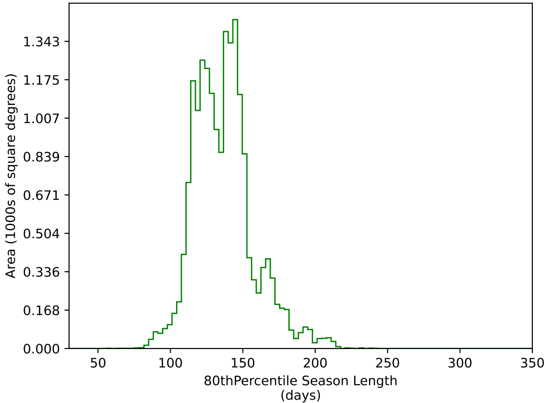
too_elab_r32_d2_giz_v3.4_10yrs WFD g band: 80thPercentile Season Length
