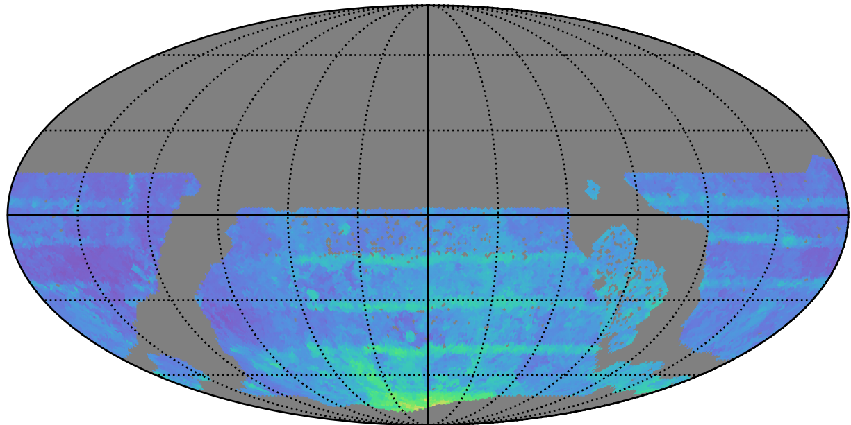
too_elab_r32_d2_giz_v3.4_10yrs WFD all bands: 80thPercentile Season Length
