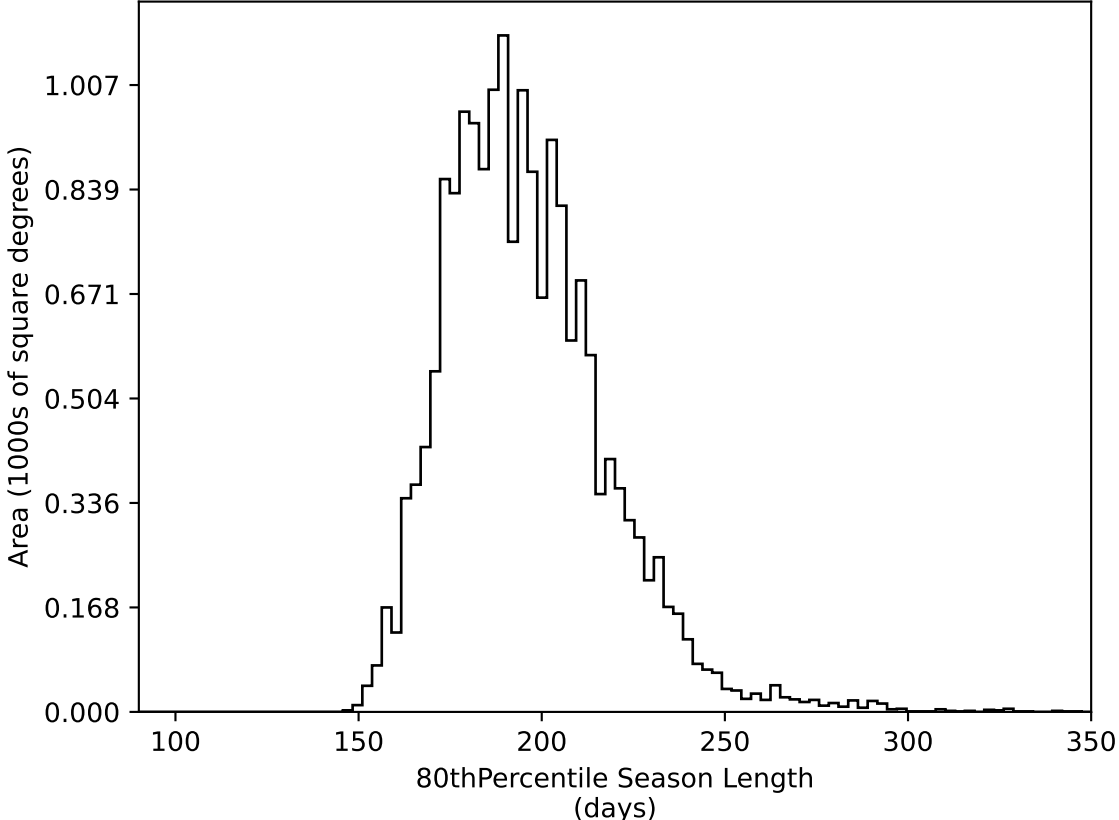
too_elab_r32_d2_giz_v3.4_10yrs WFD all bands: 80thPercentile Season Length
