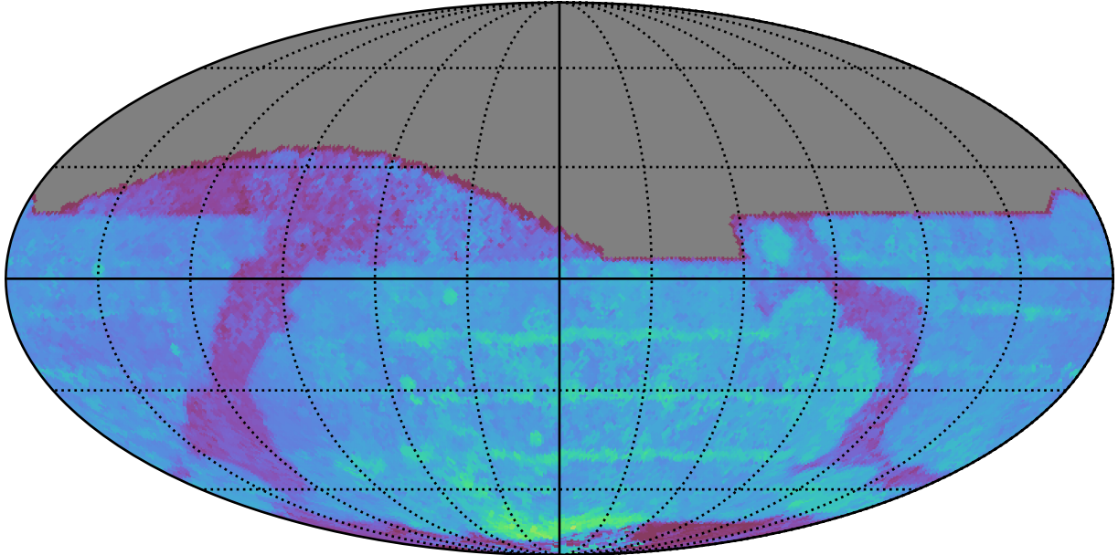
too_elab_r32_d2_giz_v3.4_10yrs All sky z band: 80thPercentile Season Length
