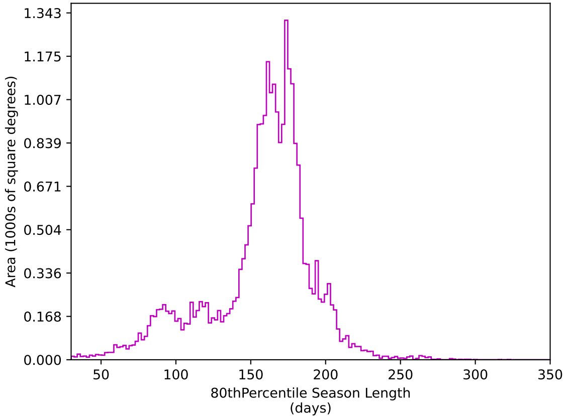
too_elab_r32_d2_giz_v3.4_10yrs All sky z band: 80thPercentile Season Length
