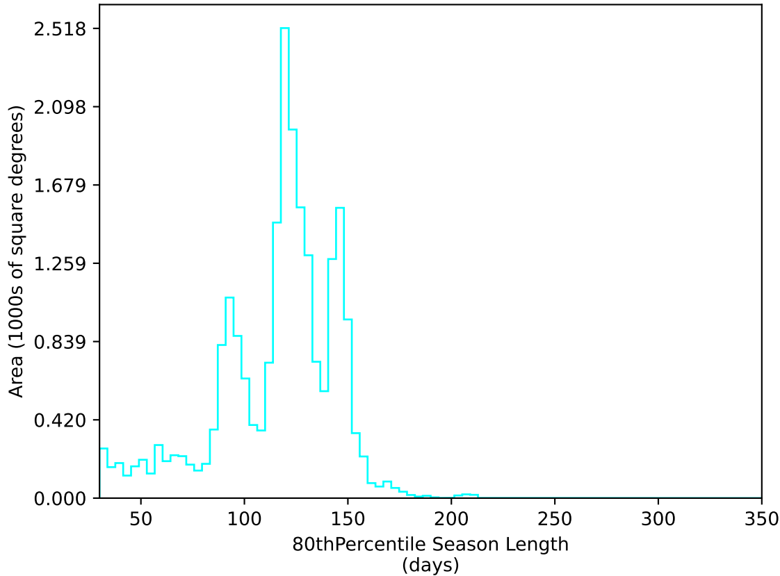
too_elab_r32_d2_giz_v3.4_10yrs All sky u band: 80thPercentile Season Length
