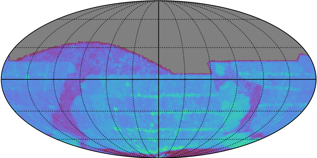
too_elab_r32_d2_giz_v3.4_10yrs All sky r band: 80thPercentile Season Length
