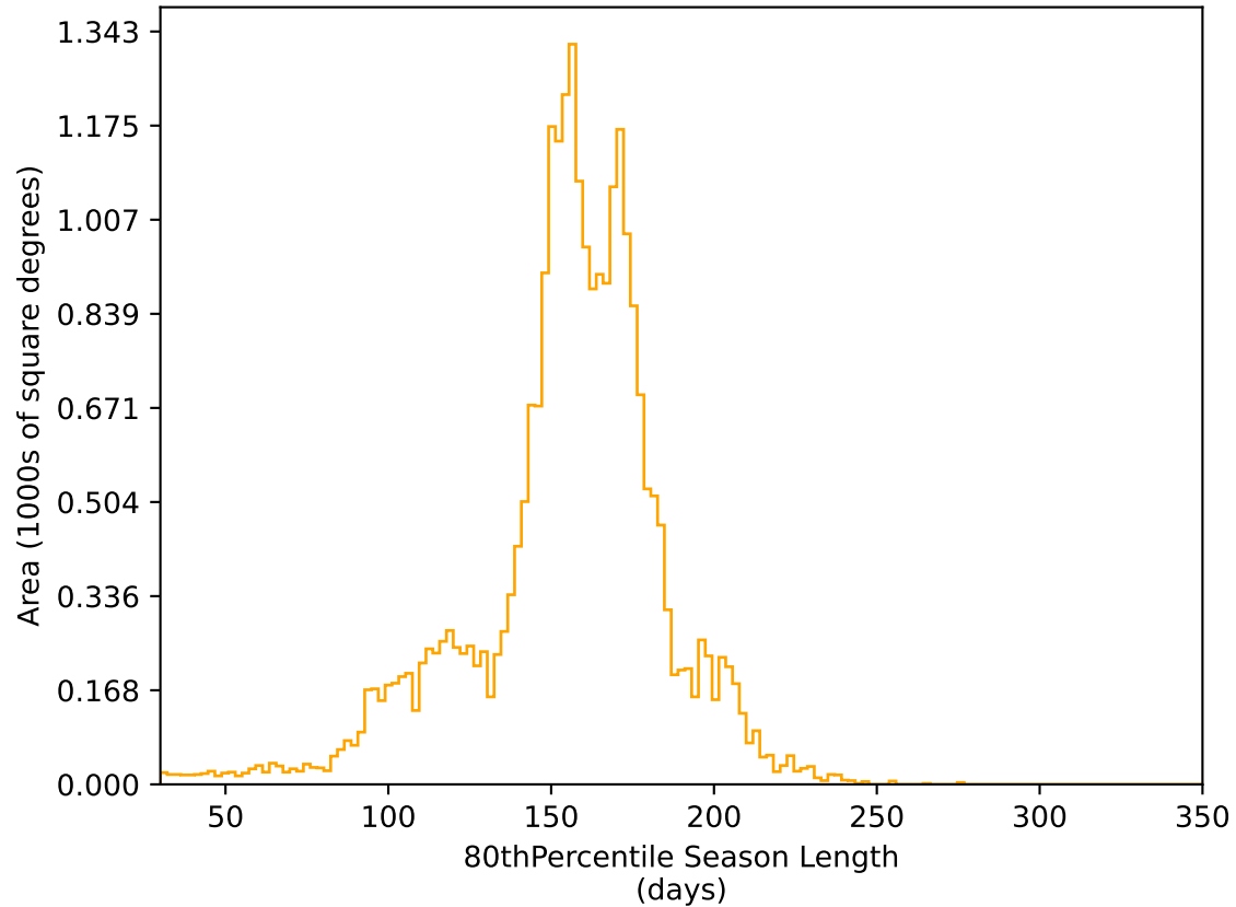
too_elab_r32_d2_giz_v3.4_10yrs All sky r band: 80thPercentile Season Length
