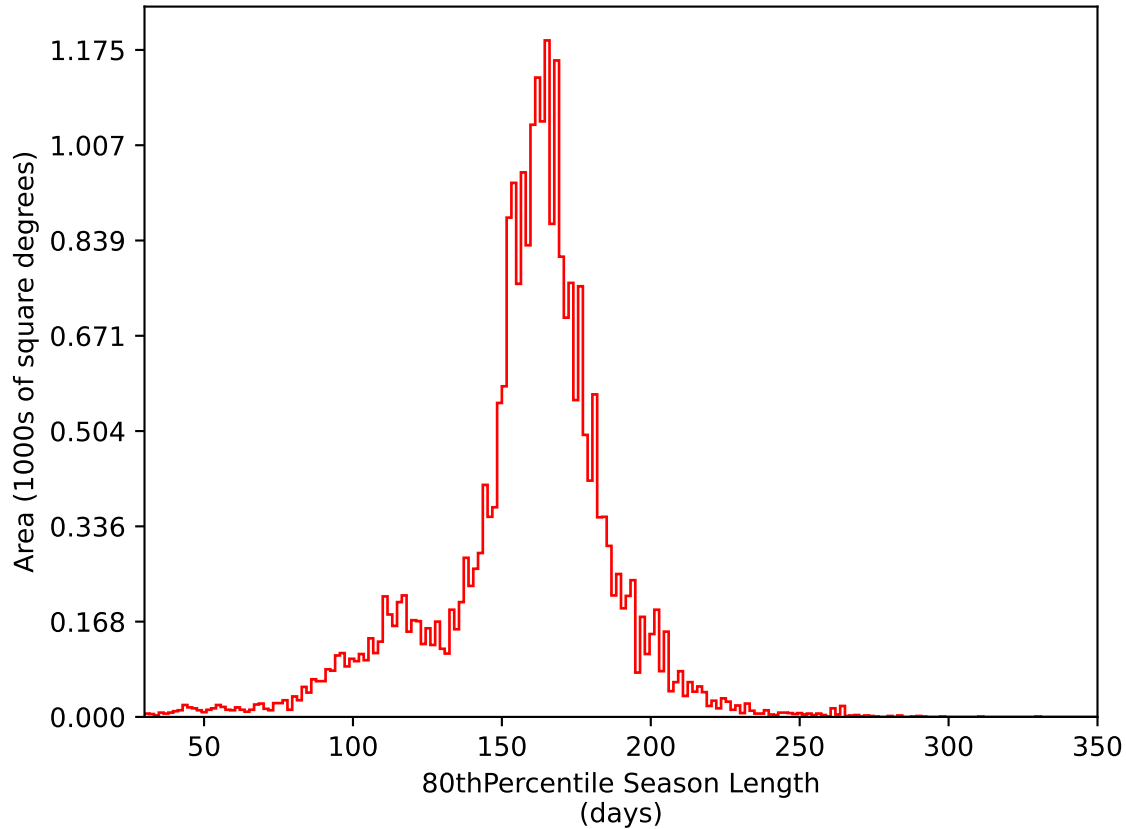
too_elab_r32_d2_giz_v3.4_10yrs All sky i band: 80thPercentile Season Length
