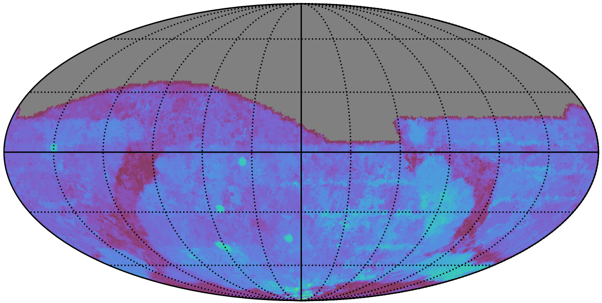
too_elab_r32_d2_giz_v3.4_10yrs All sky g band: 80thPercentile Season Length
