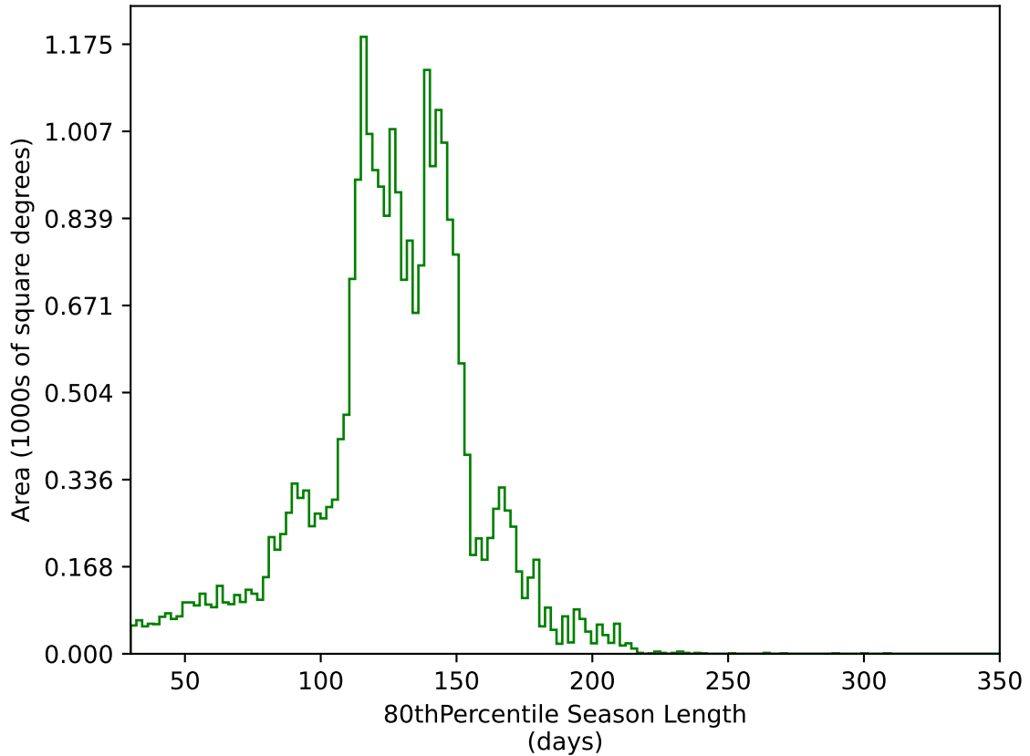
too_elab_r32_d2_giz_v3.4_10yrs All sky g band: 80thPercentile Season Length
