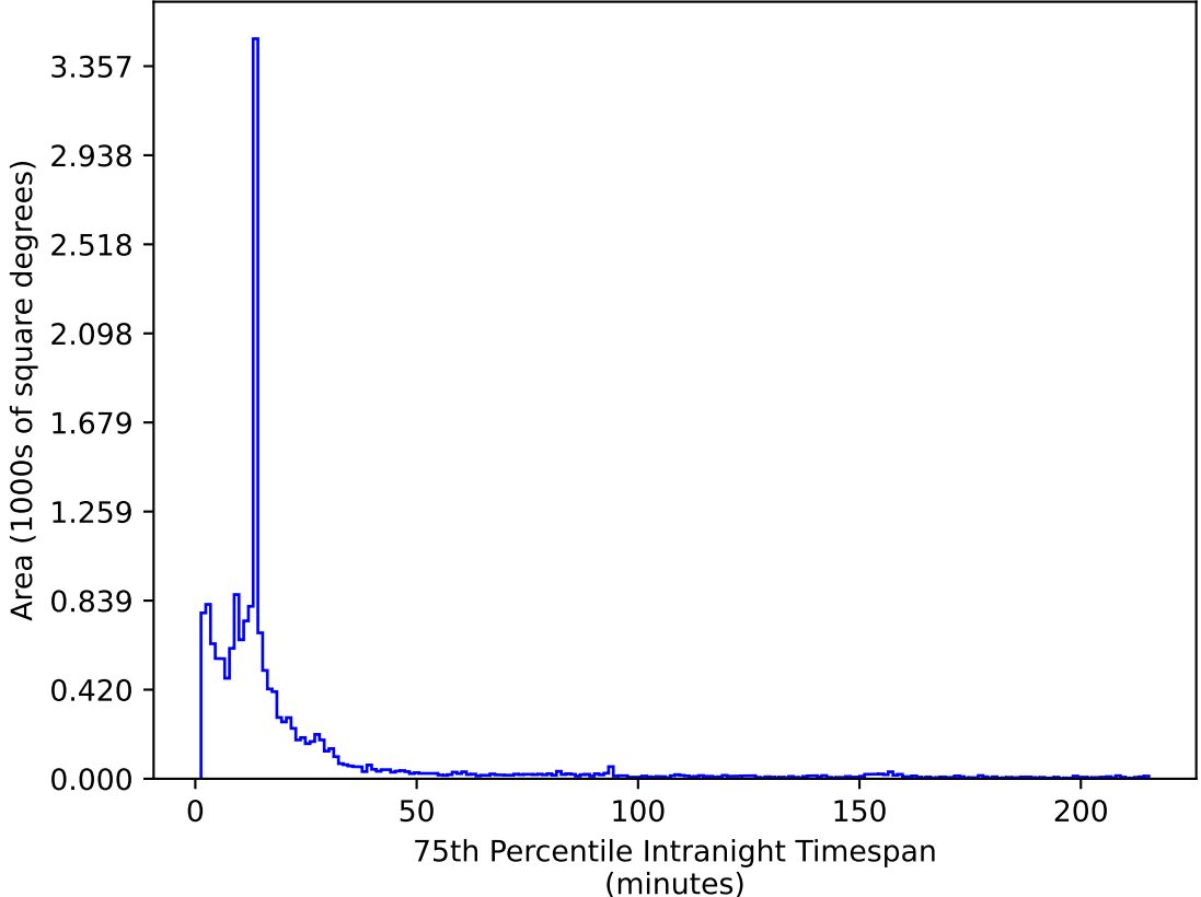
too_elab_r32_d2_giz_v3.4_10yrs WFD z band: 75th Percentile Intranight Timespan
