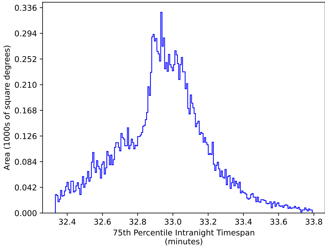
too_elab_r32_d2_giz_v3.4_10yrs WFD y band: 75th Percentile Intranight Timespan
