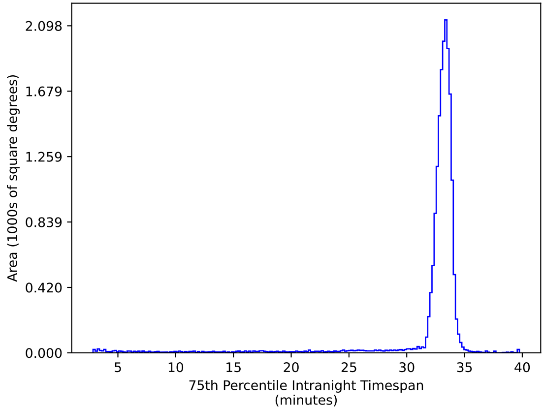
too_elab_r32_d2_giz_v3.4_10yrs WFD ug bands: 75th Percentile Intranight Timespan
