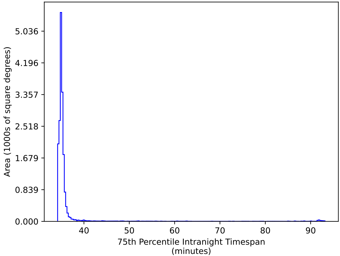
too_elab_r32_d2_giz_v3.4_10yrs WFD ri bands: 75th Percentile Intranight Timespan
