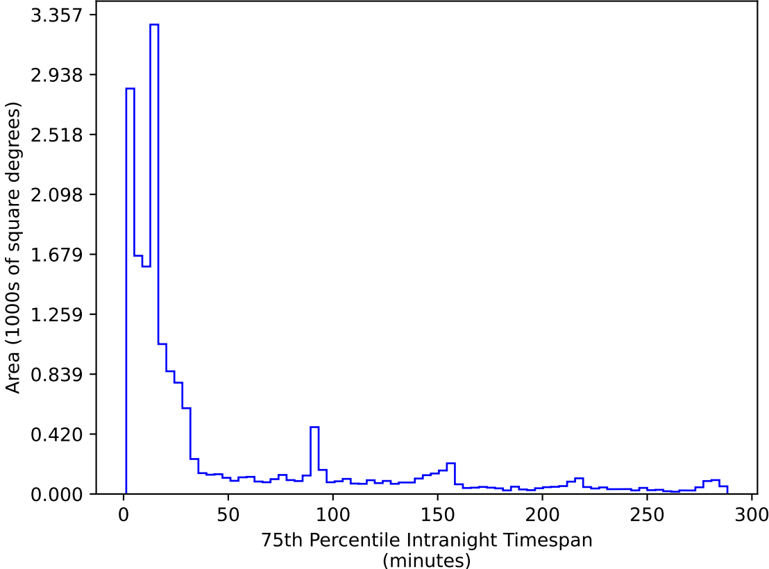
too_elab_r32_d2_giz_v3.4_10yrs WFD r band: 75th Percentile Intranight Timespan
