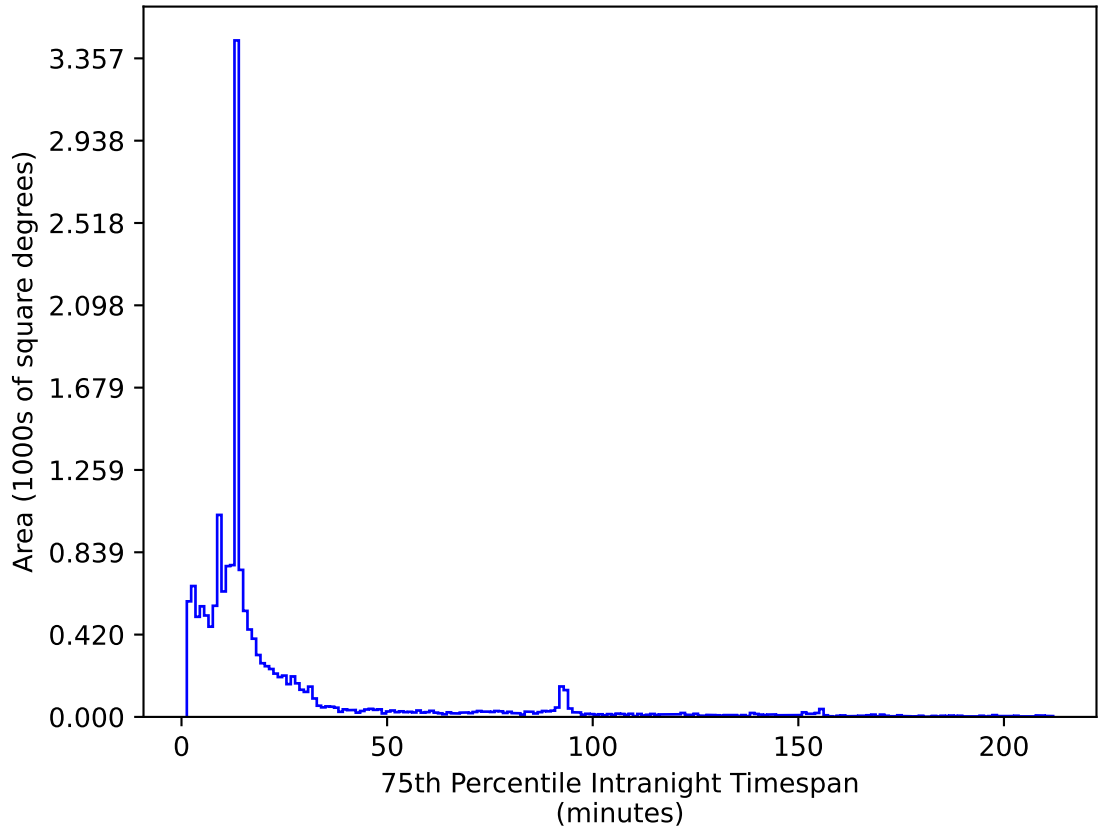
too_elab_r32_d2_giz_v3.4_10yrs WFD i band: 75th Percentile Intranight Timespan
