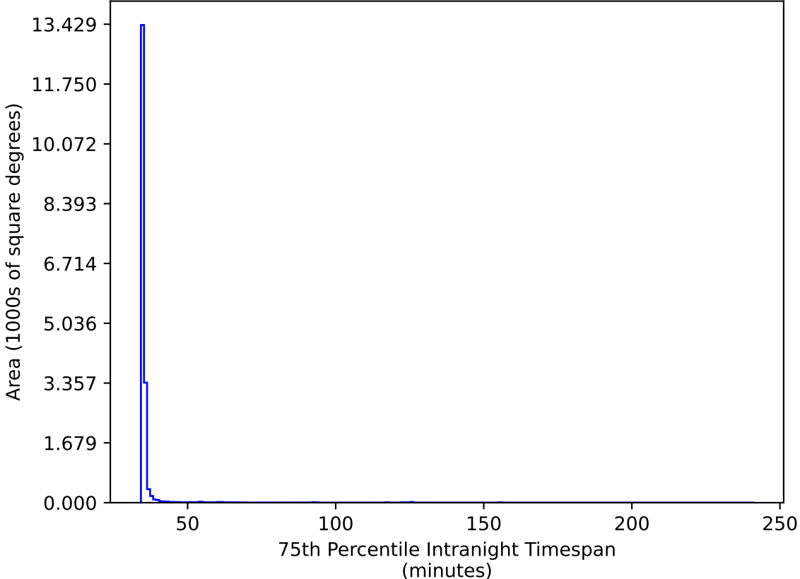
too_elab_r32_d2_giz_v3.4_10yrs WFD gr bands: 75th Percentile Intranight Timespan
